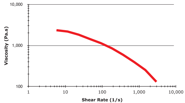
Shear-Viscosity @ 190 °C
